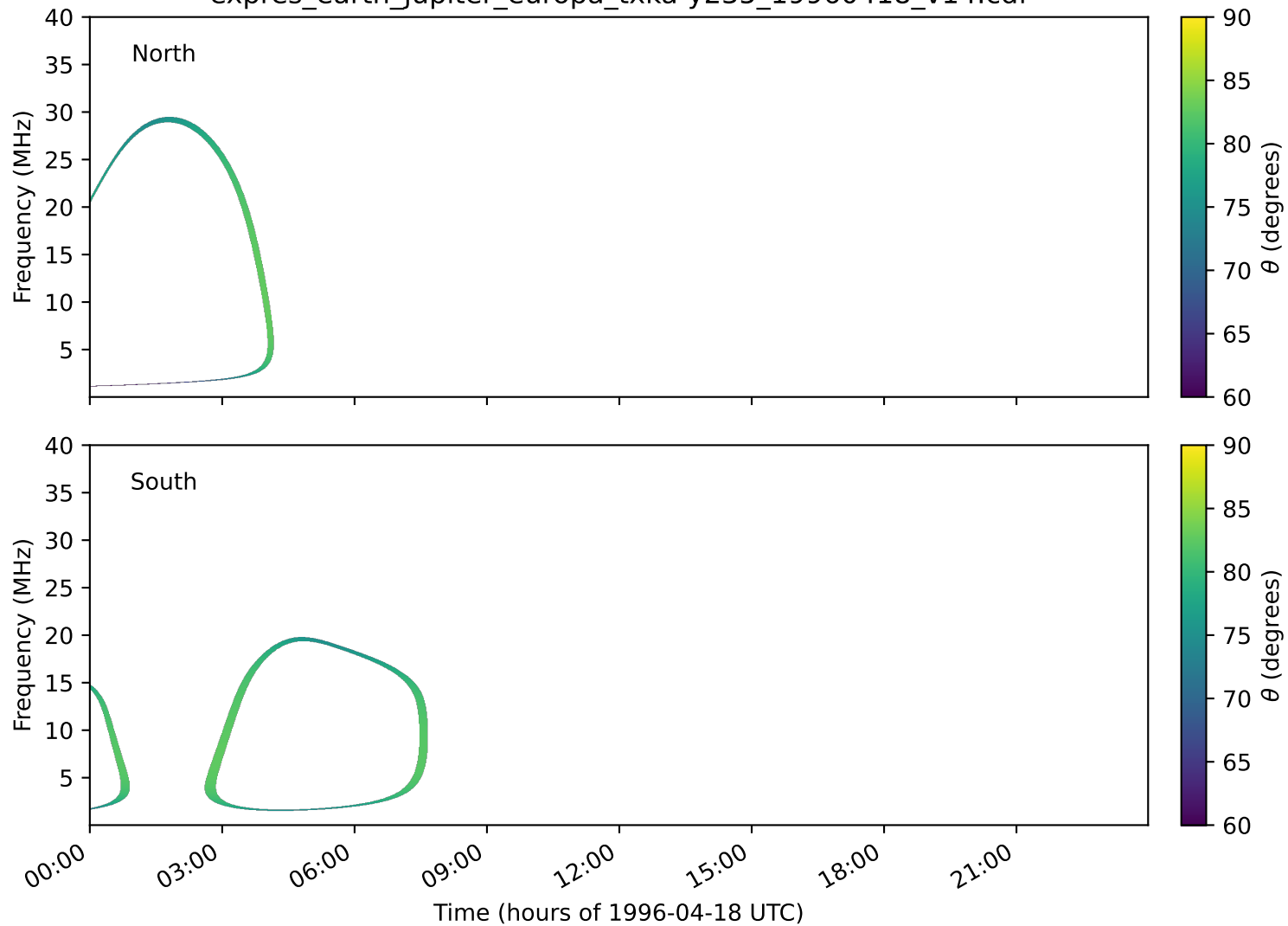
expres_earth_jupiter_europa_txka-y235_19960418_v14.cdf
