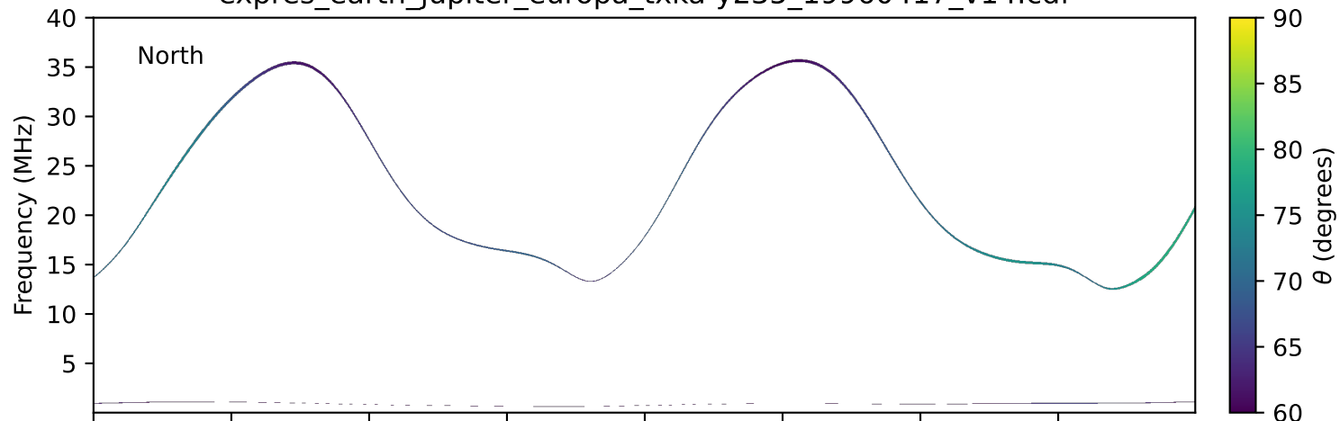
expres_earth_jupiter_europa_txka-y235_19960417_v14.cdf
