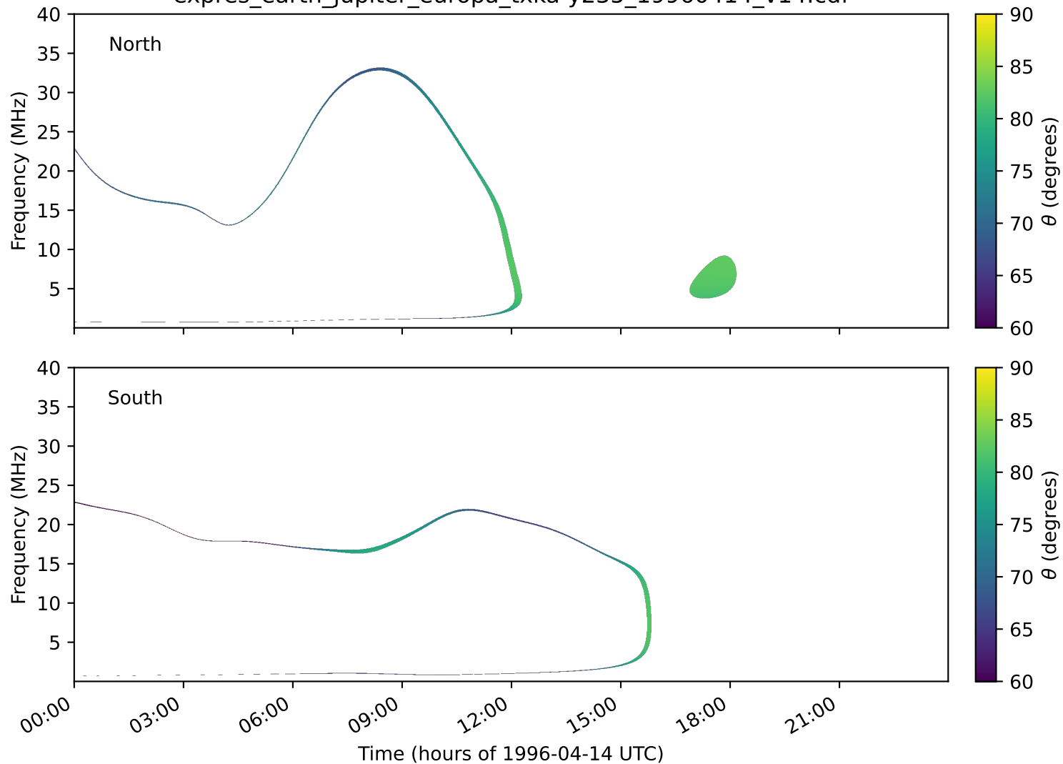
expres_earth_jupiter_europa_txka-y235_19960414_v14.cdf
