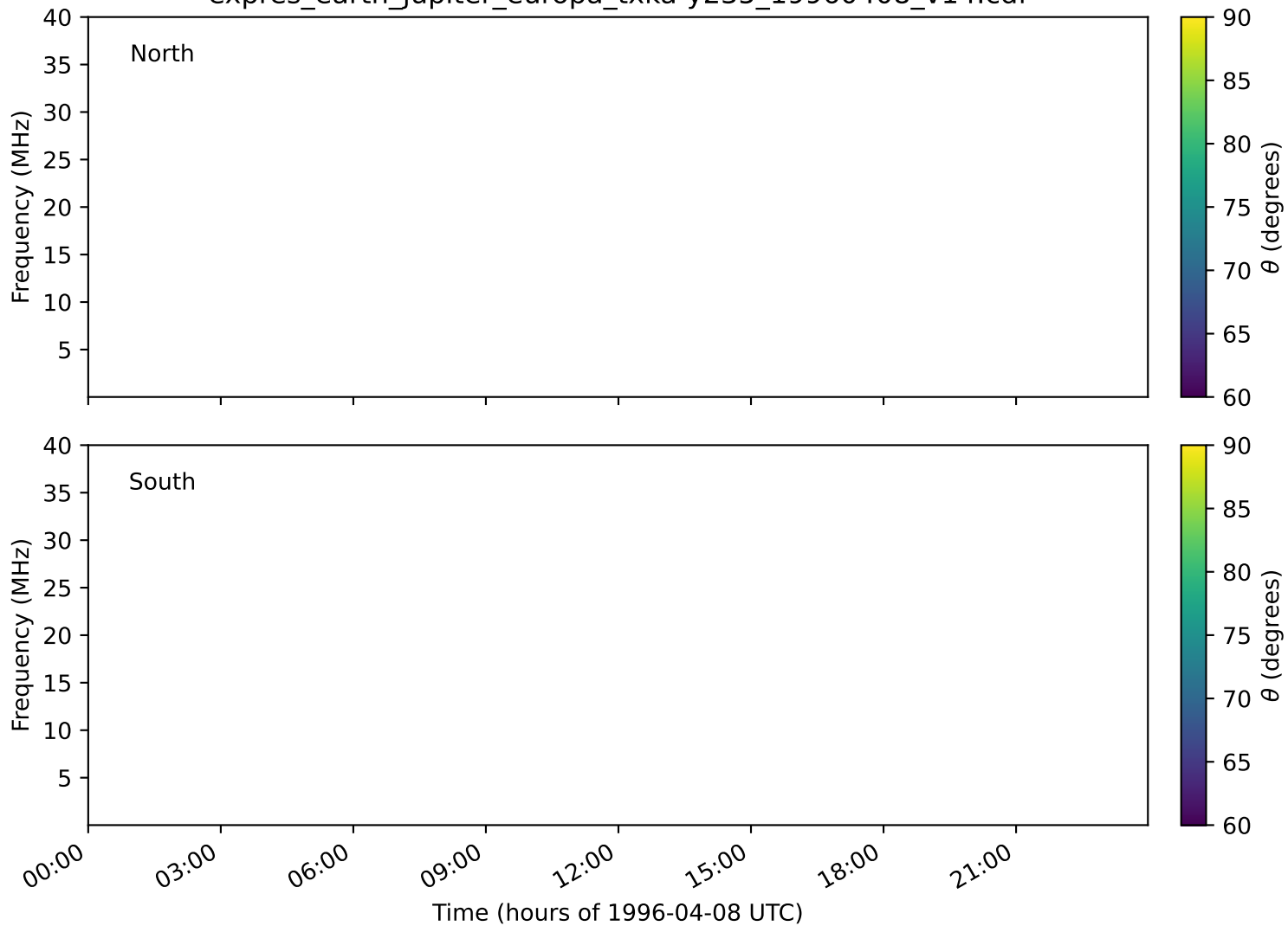
expres_earth_jupiter_europa_txka-y235_19960408_v14.cdf
