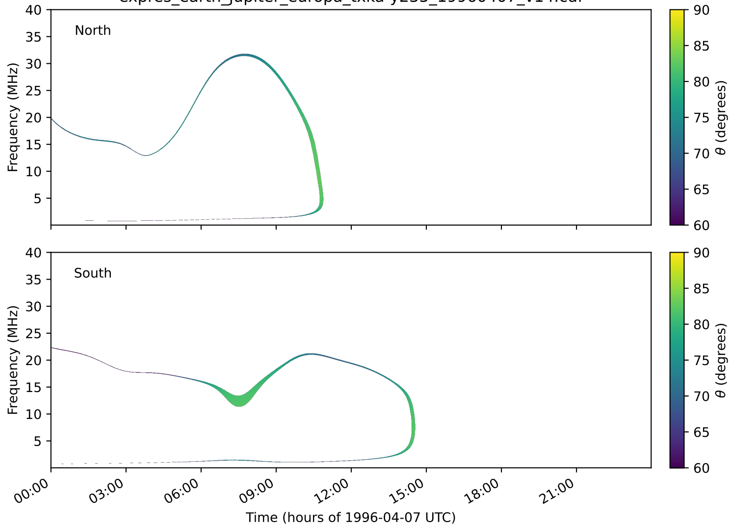
expres_earth_jupiter_europa_txka-y235_19960407_v14.cdf
