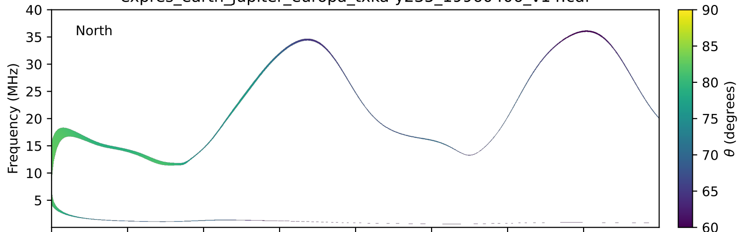
expres_earth_jupiter_europa_txka-y235_19960406_v14.cdf
