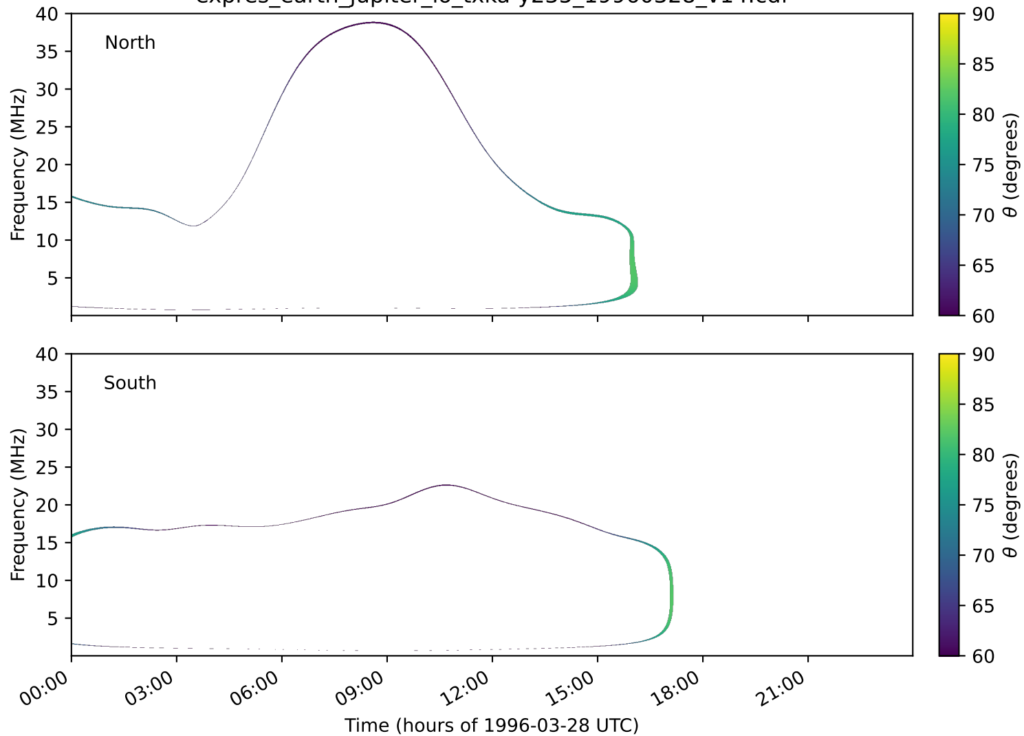
expres_earth_jupiter_io_txka-y235_19960328_v14.cdf
