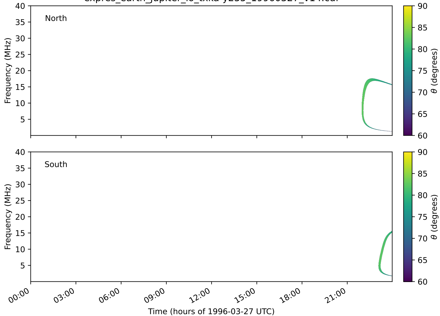
expres_earth_jupiter_io_txka-y235_19960327_v14.cdf
