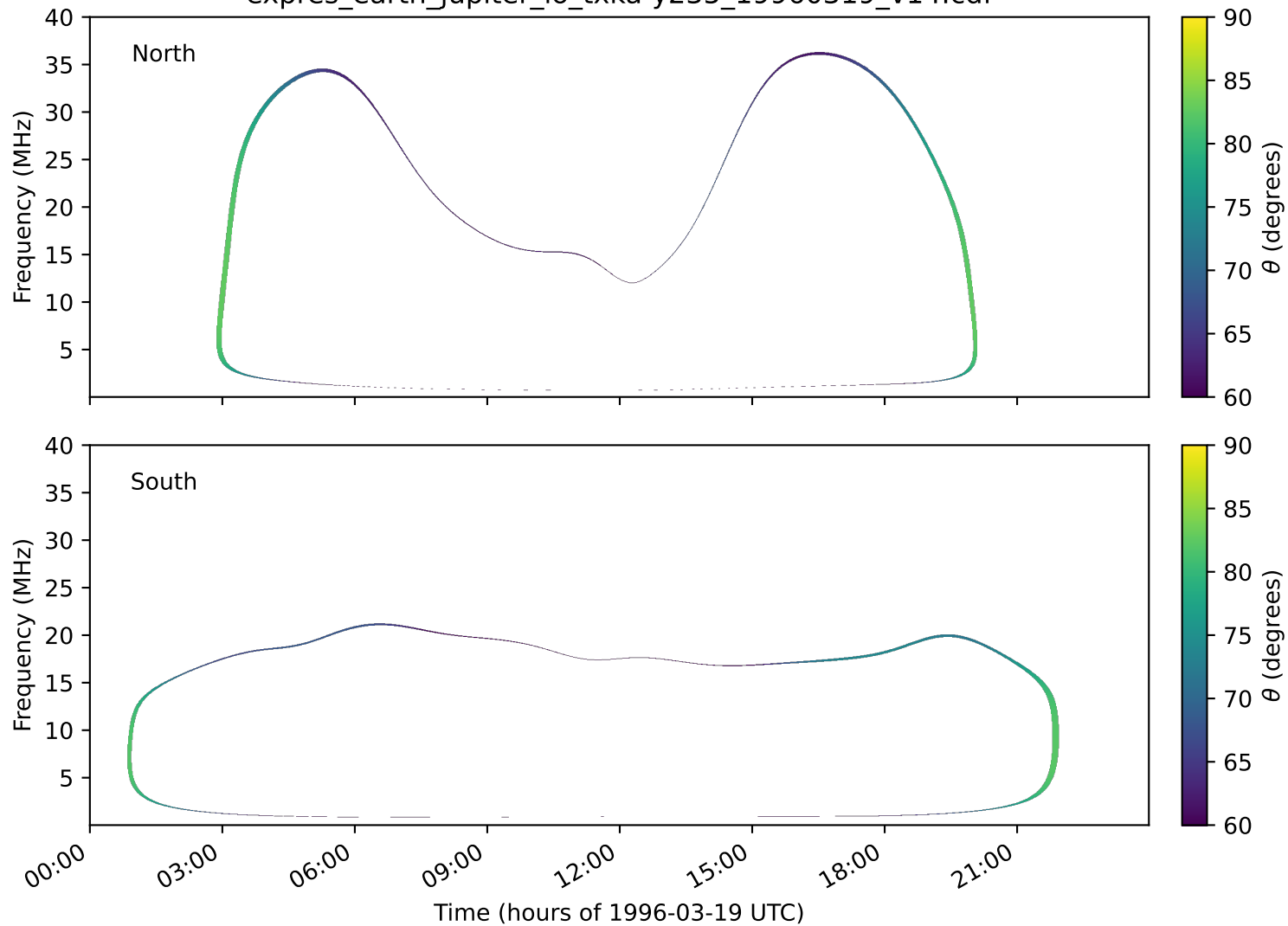
expres_earth_jupiter_io_txka-y235_19960319_v14.cdf
