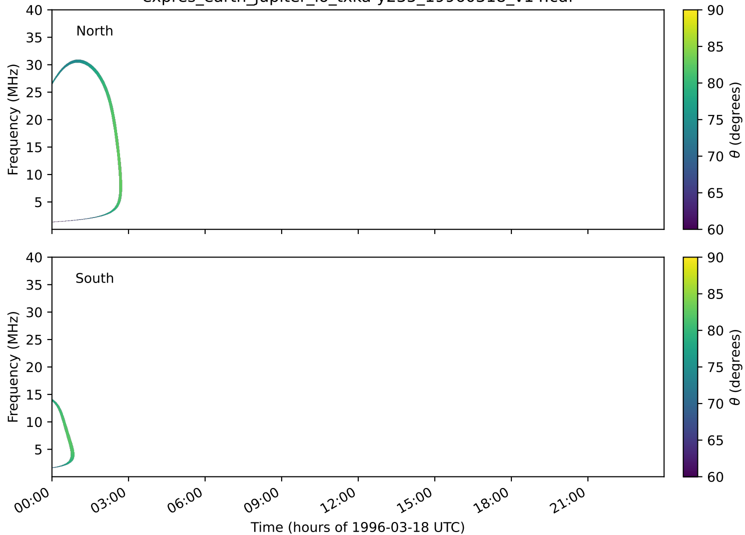
expres_earth_jupiter_io_txka-y235_19960318_v14.cdf
