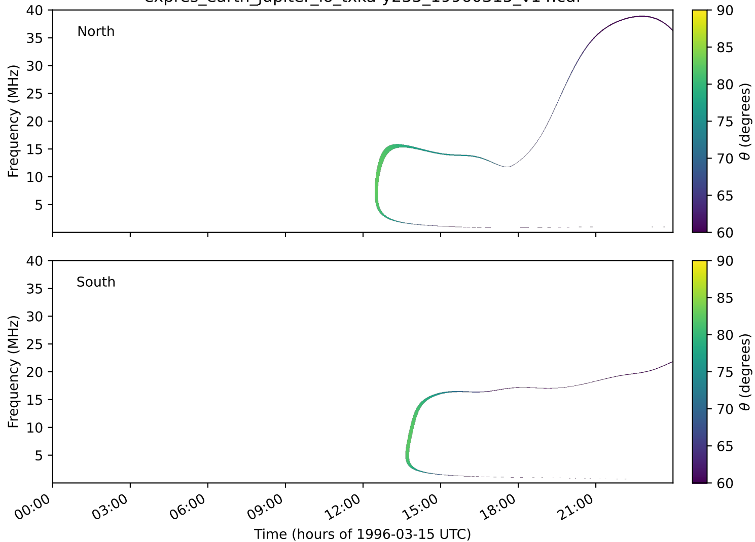
expres_earth_jupiter_io_txka-y235_19960315_v14.cdf
