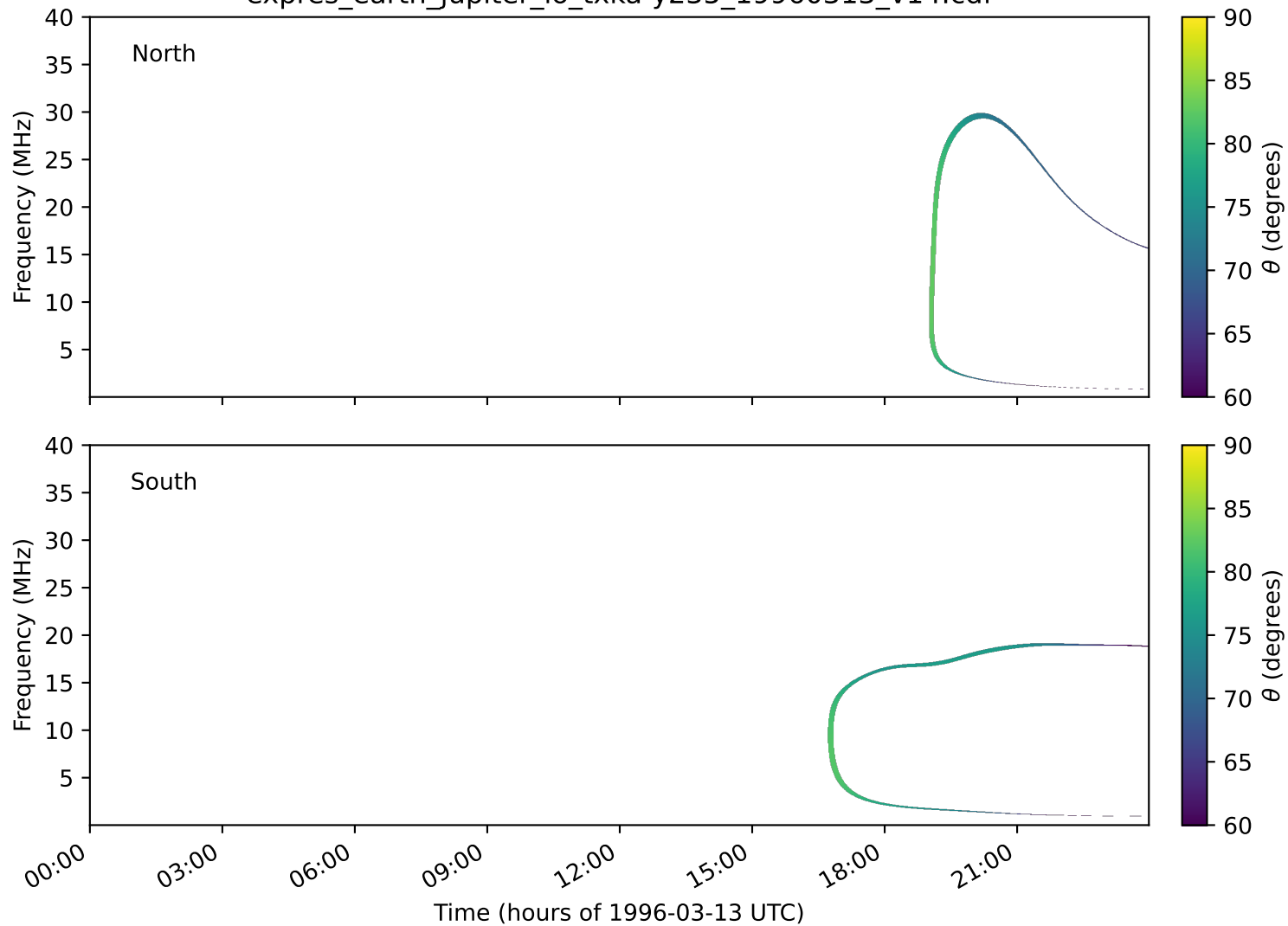
expres_earth_jupiter_io_txka-y235_19960313_v14.cdf
