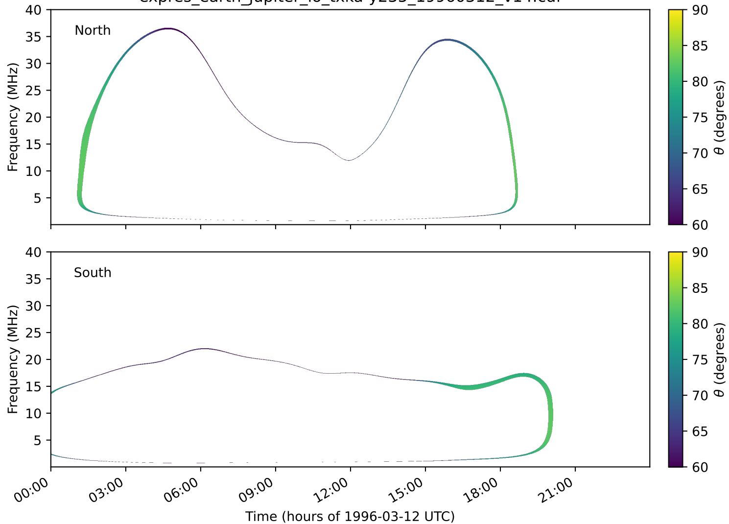
expres_earth_jupiter_io_txka-y235_19960312_v14.cdf
