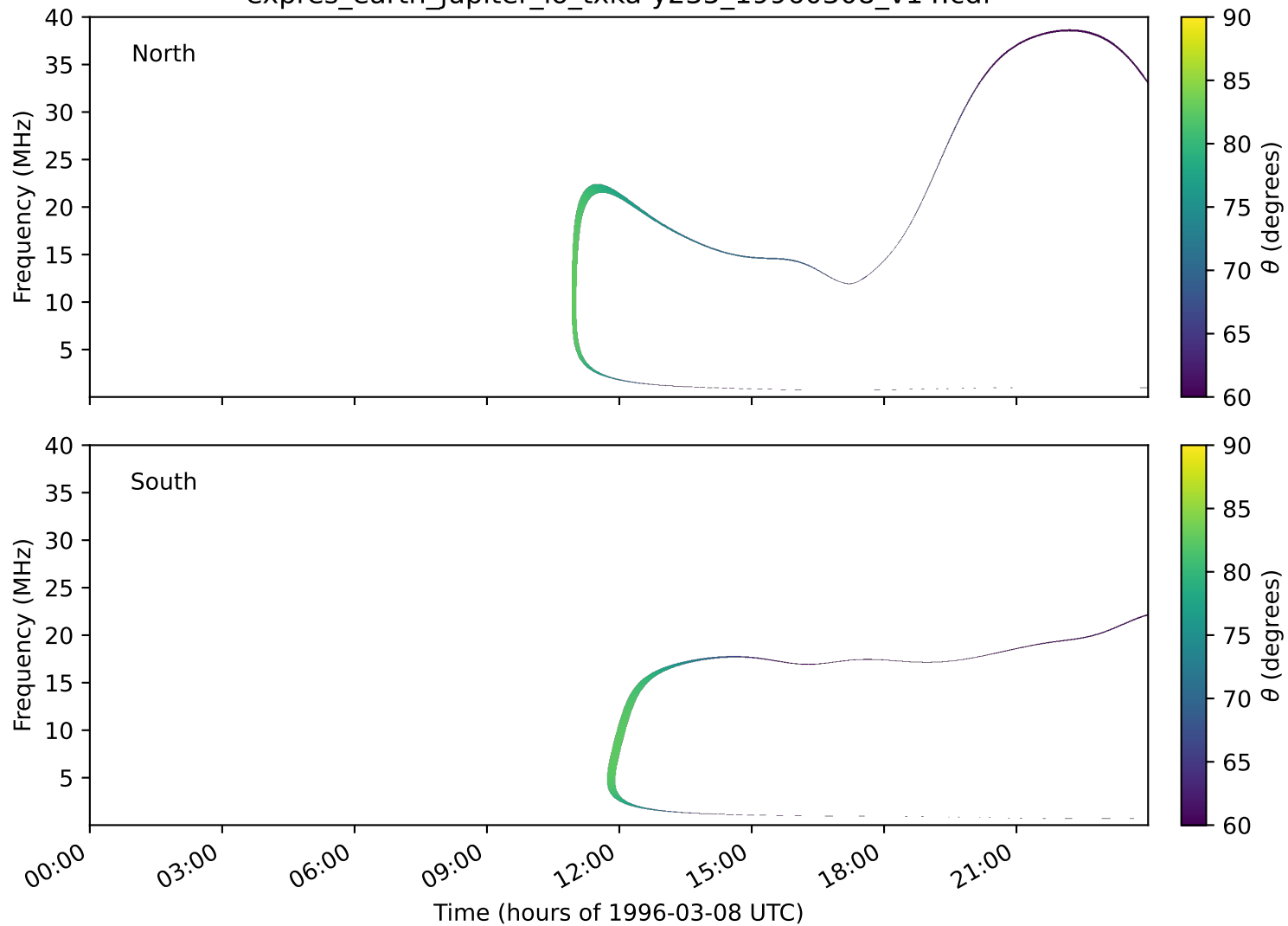
expres_earth_jupiter_io_txka-y235_19960308_v14.cdf
