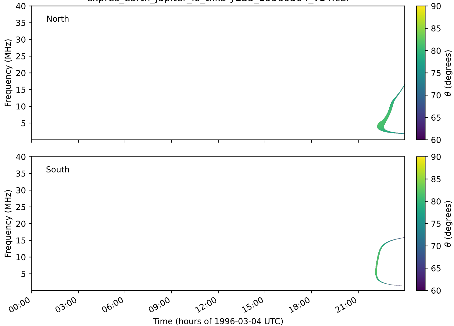
expres_earth_jupiter_io_txka-y235_19960304_v14.cdf
