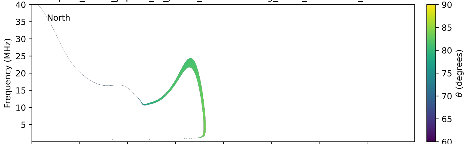
expres_earth_jupiter_io_jrm33_lossc-wid1deg_3kev_19960323_v11.cdf
