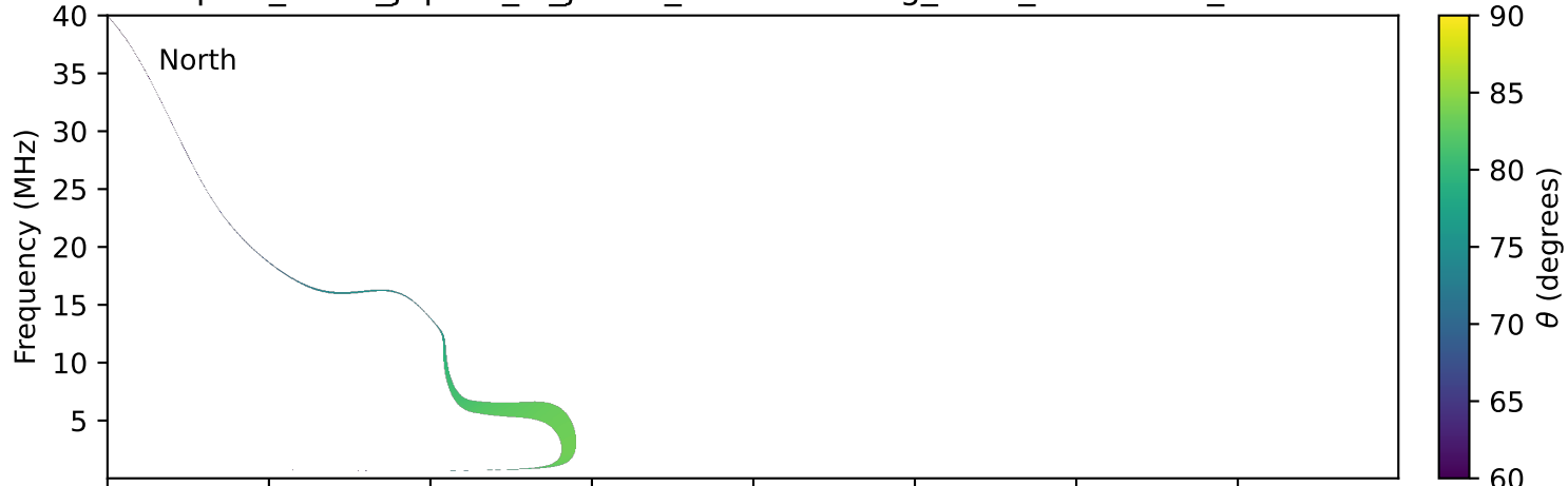
expres_earth_jupiter_io_jrm33_lossc-wid1deg_3kev_19960316_v11.cdf
