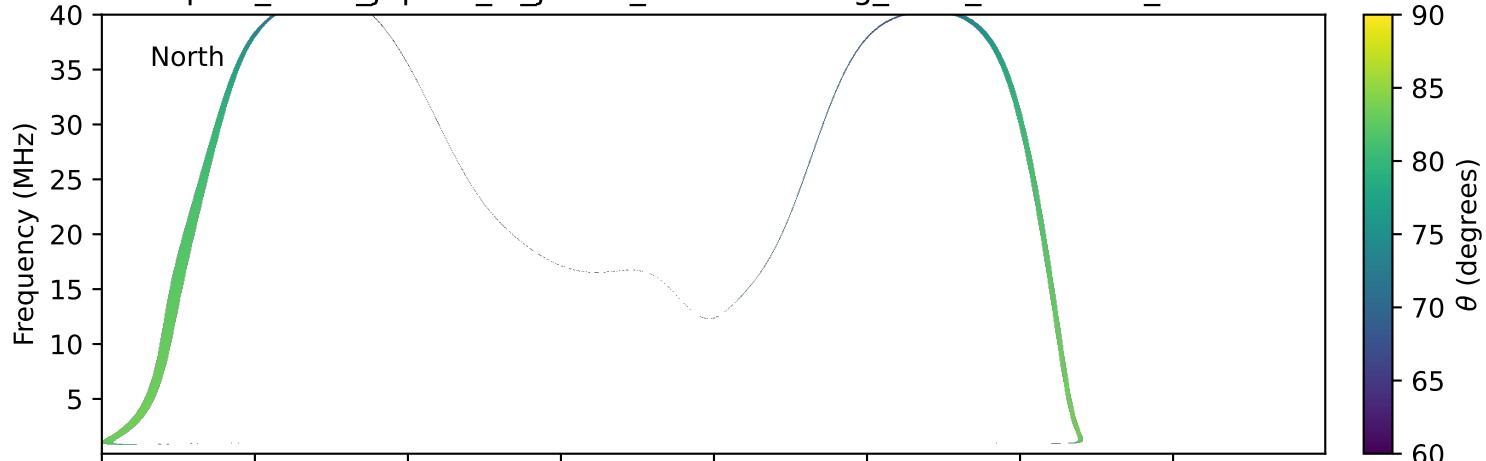
expres_earth_jupiter_io_jrm33_lossc-wid1deg_3kev_19960312_v11.cdf
