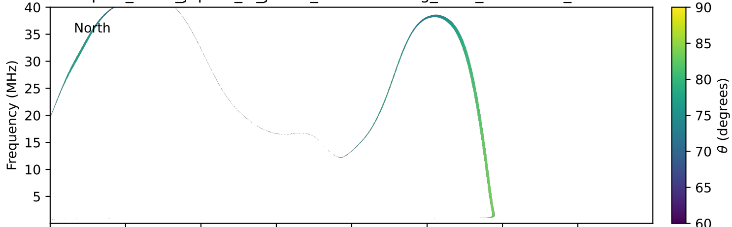
expres_earth_jupiter_io_jrm33_lossc-wid1deg_3kev_19960305_v11.cdf
