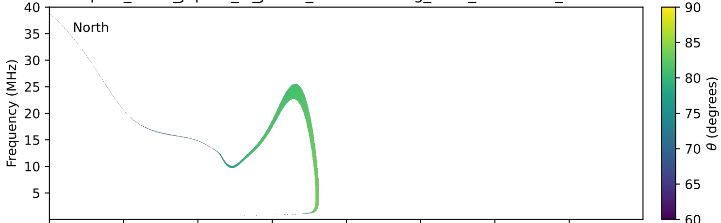
expres_earth_jupiter_io_jrm09_lossc-wid1deg_3kev_19960323_v11.cdf
