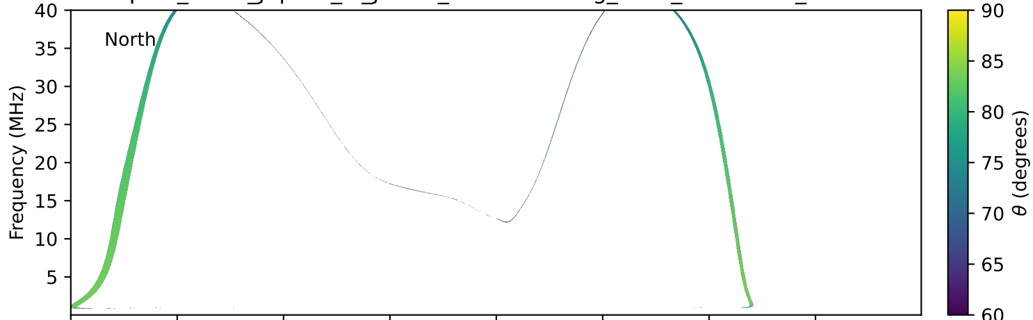
expres_earth_jupiter_io_jrm09_lossc-wid1deg_3kev_19960312_v11.cdf
