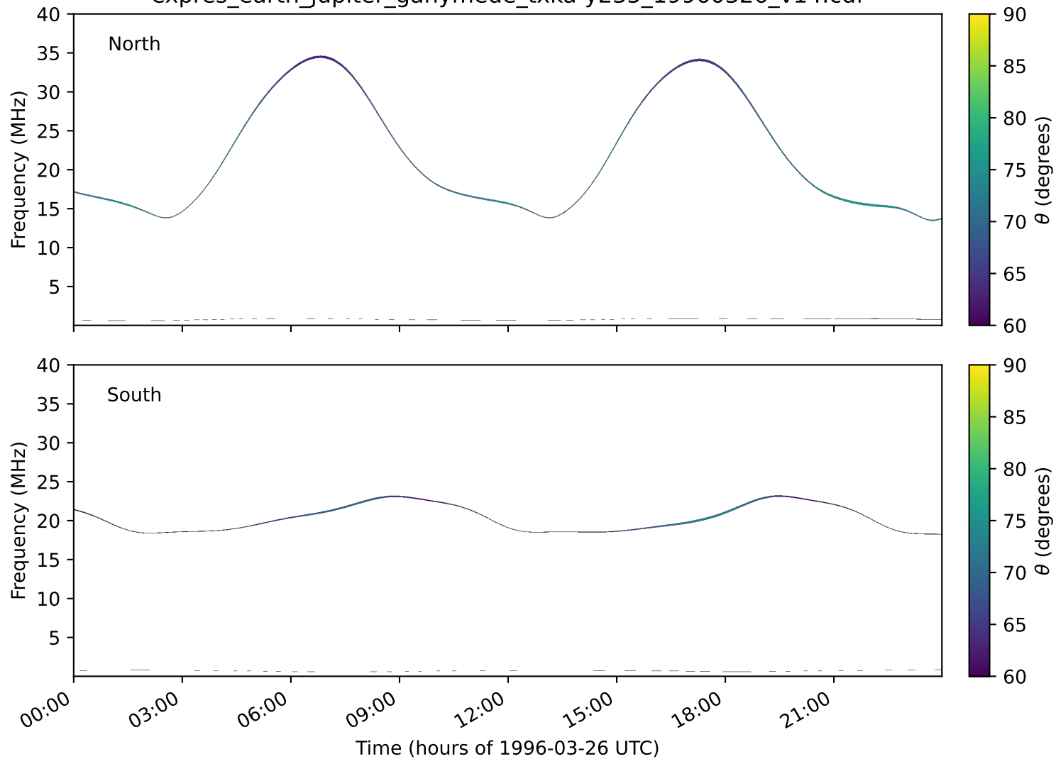
expres_earth_jupiter_ganymede_txka-y235_19960326_v14.cdf
