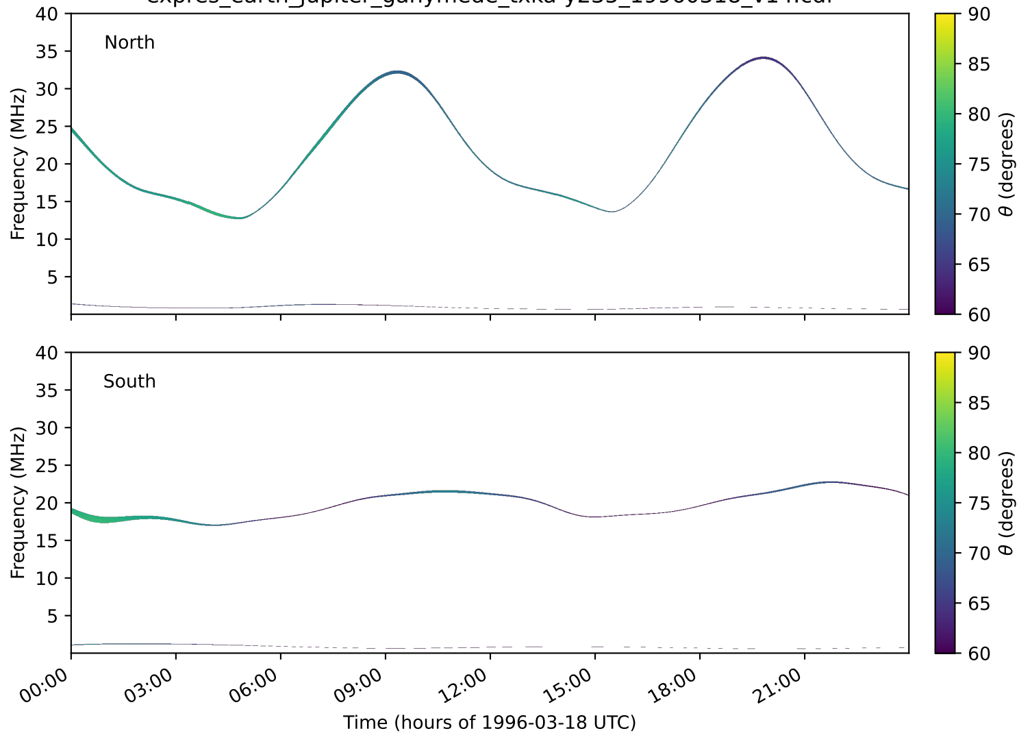
expres_earth_jupiter_ganymede_txka-y235_19960318_v14.cdf
