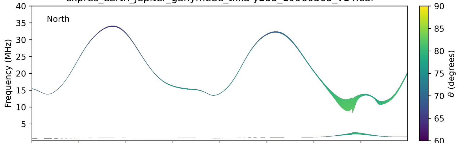
expres_earth_jupiter_ganymede_txka-y235_19960305_v14.cdf
