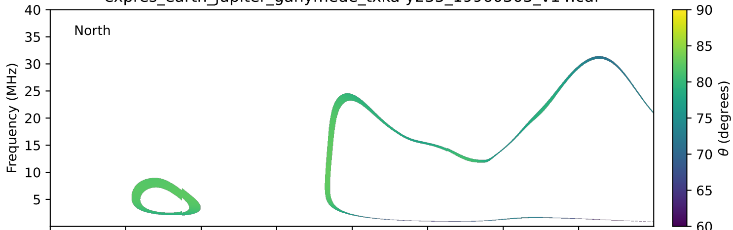
expres_earth_jupiter_ganymede_txka-y235_19960303_v14.cdf
