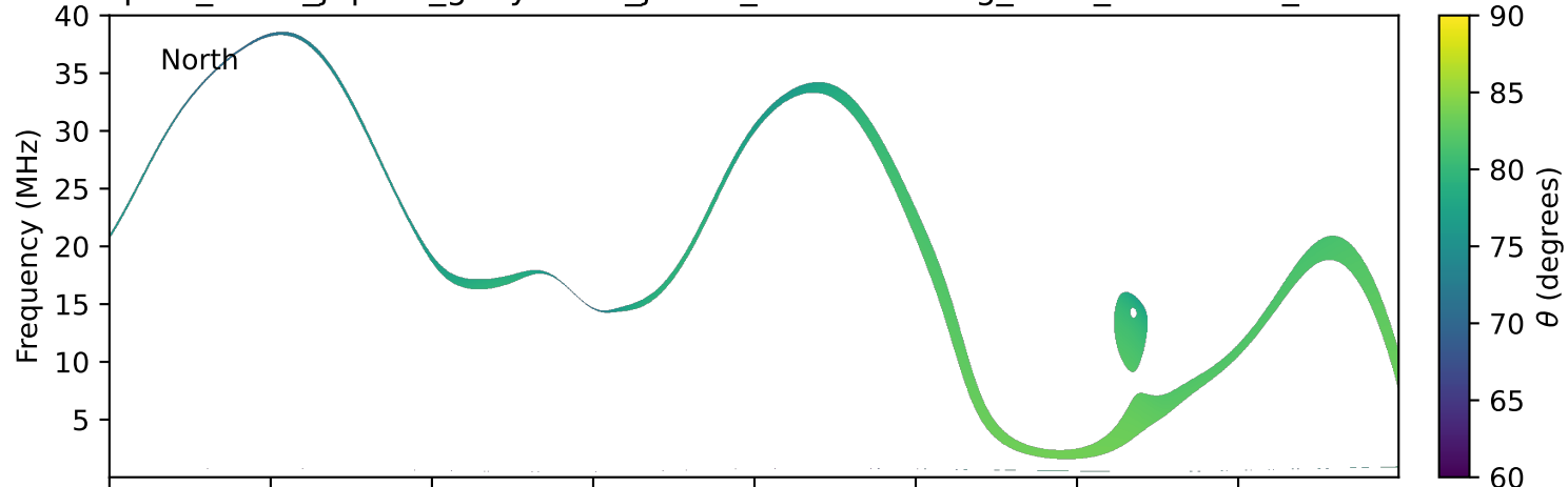
expres_earth_jupiter_ganymede_jrm33_lossc-wid1deg_3kev_19960320_v11.cdf
