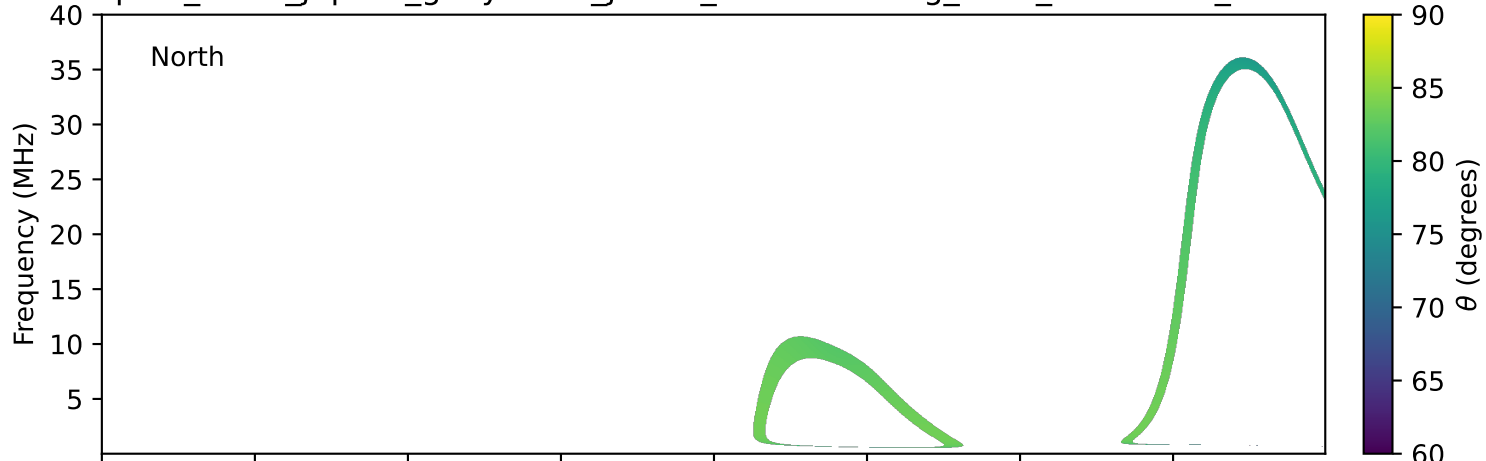
expres_earth_jupiter_ganymede_jrm33_lossc-wid1deg_3kev_19960310_v11.cdf
