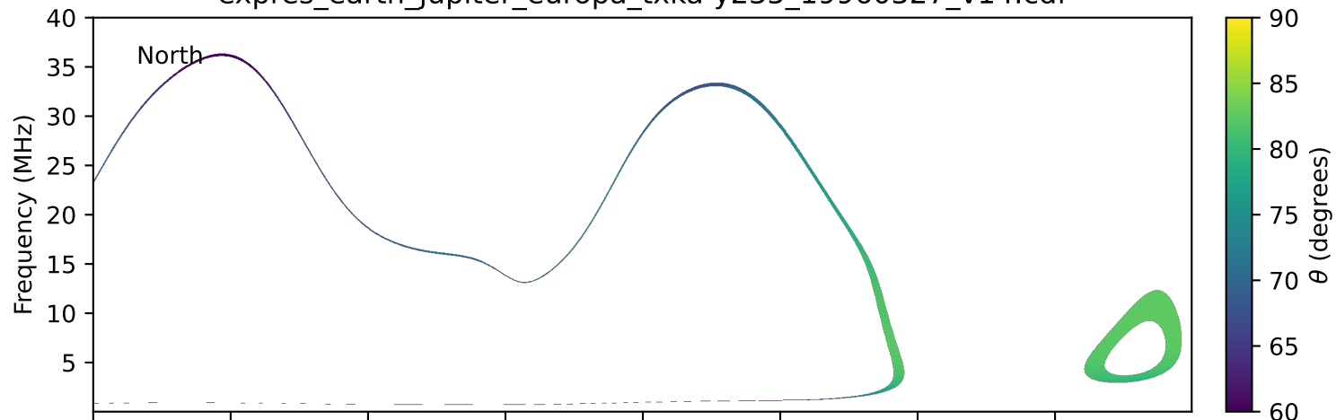
expres_earth_jupiter_europa_txka-y235_19960327_v14.cdf
