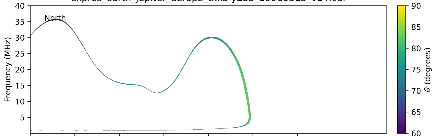
expres_earth_jupiter_europa_txka-y235_19960313_v14.cdf
