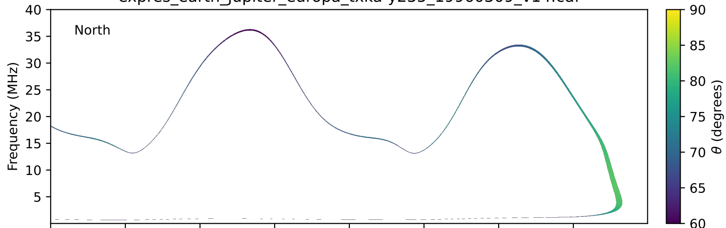
expres_earth_jupiter_europa_txka-y235_19960309_v14.cdf
