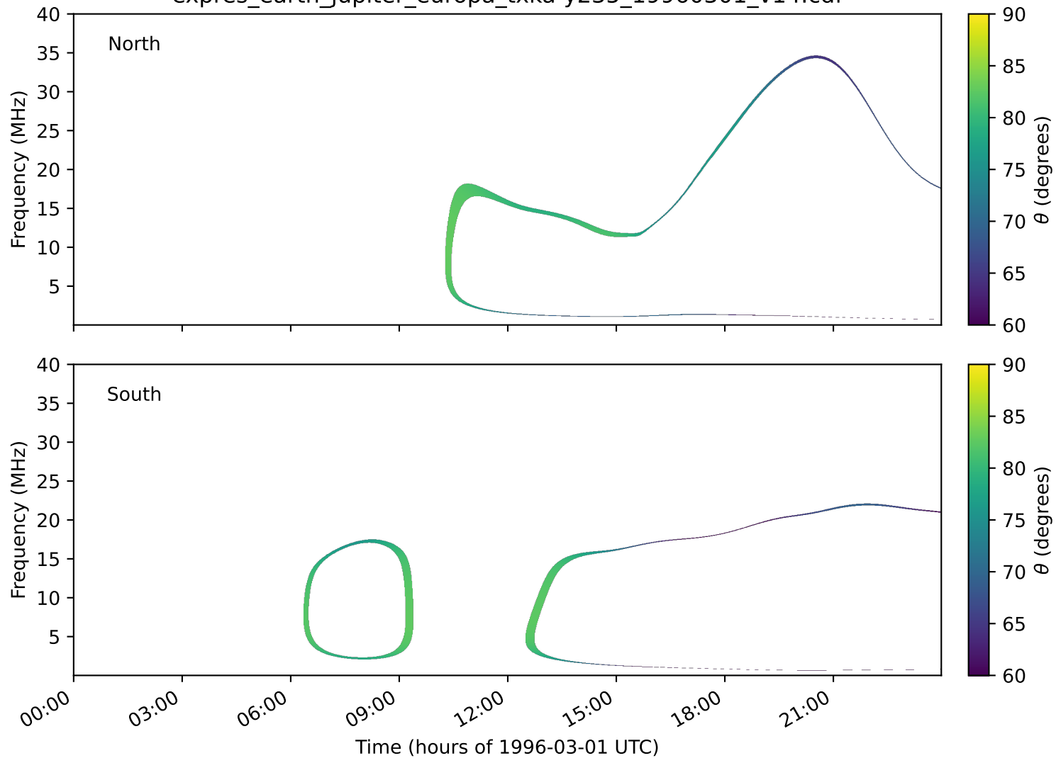
expres_earth_jupiter_europa_txka-y235_19960301_v14.cdf
