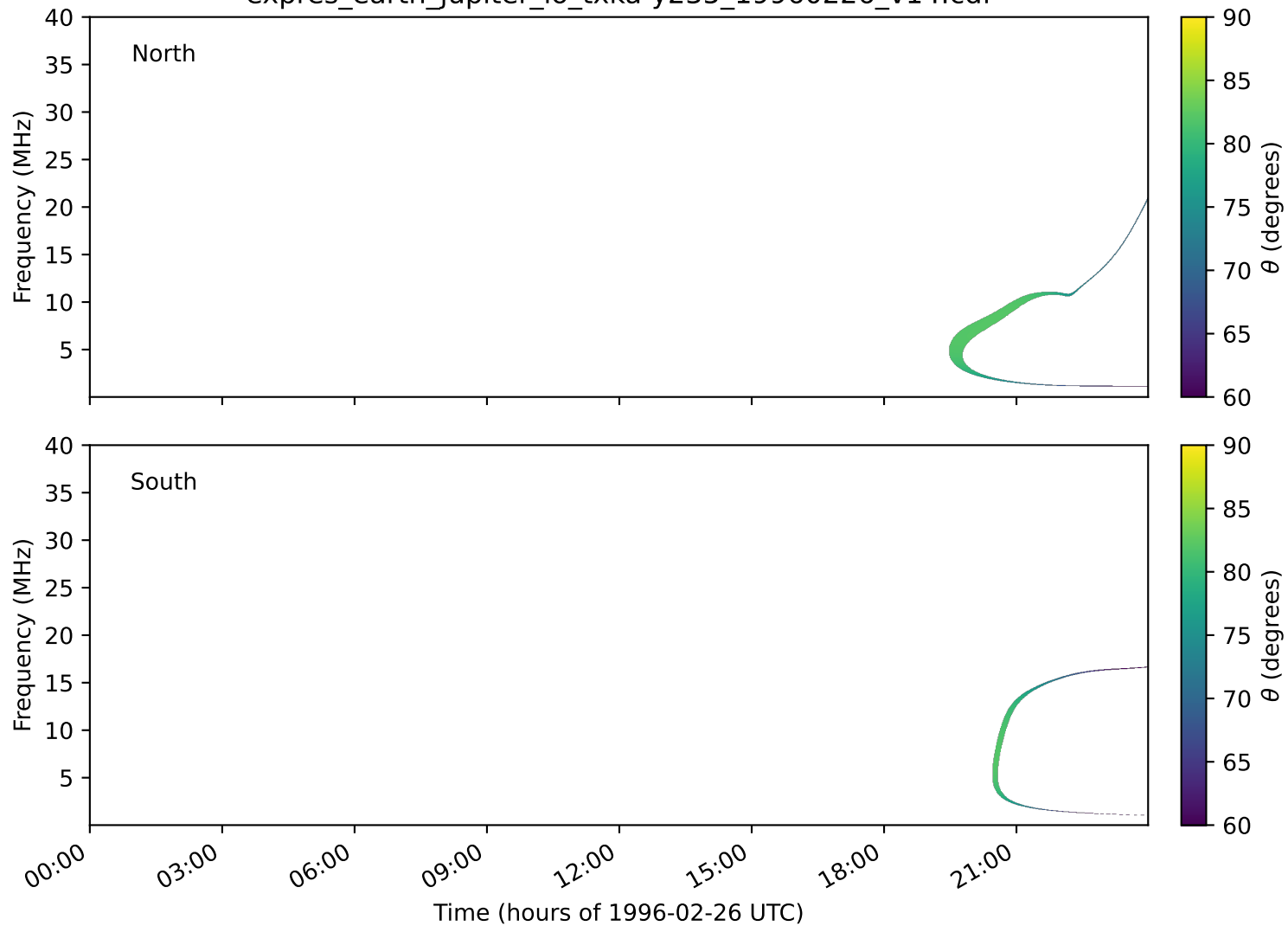
expres_earth_jupiter_io_txka-y235_19960226_v14.cdf
