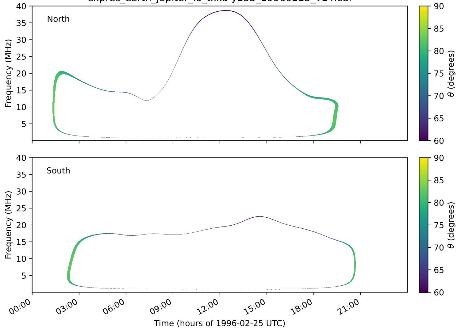
expres_earth_jupiter_io_txka-y235_19960225_v14.cdf
