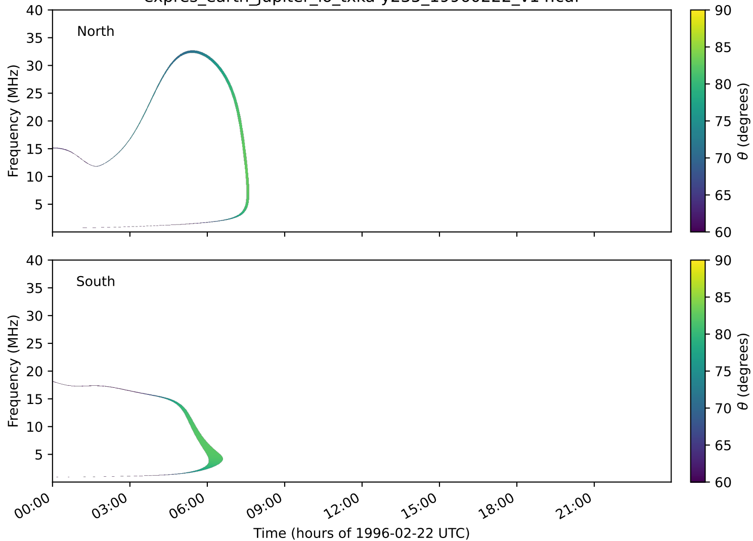
expres_earth_jupiter_io_txka-y235_19960222_v14.cdf
