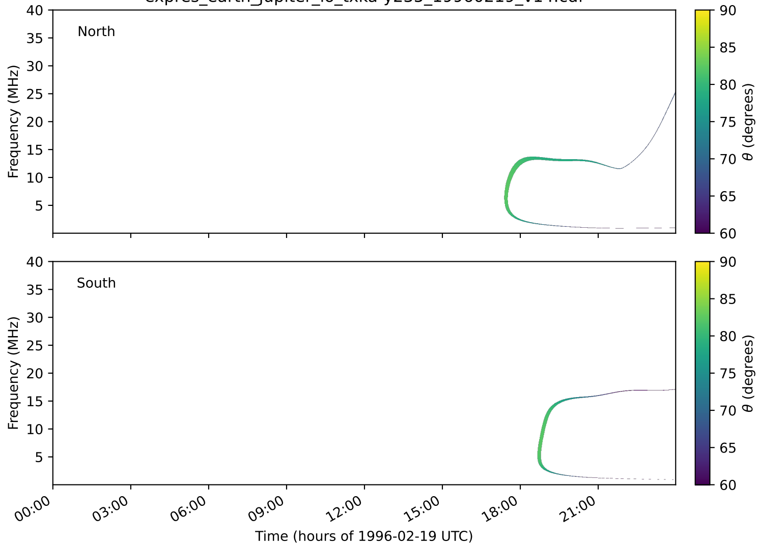
expres_earth_jupiter_io_txka-y235_19960219_v14.cdf
