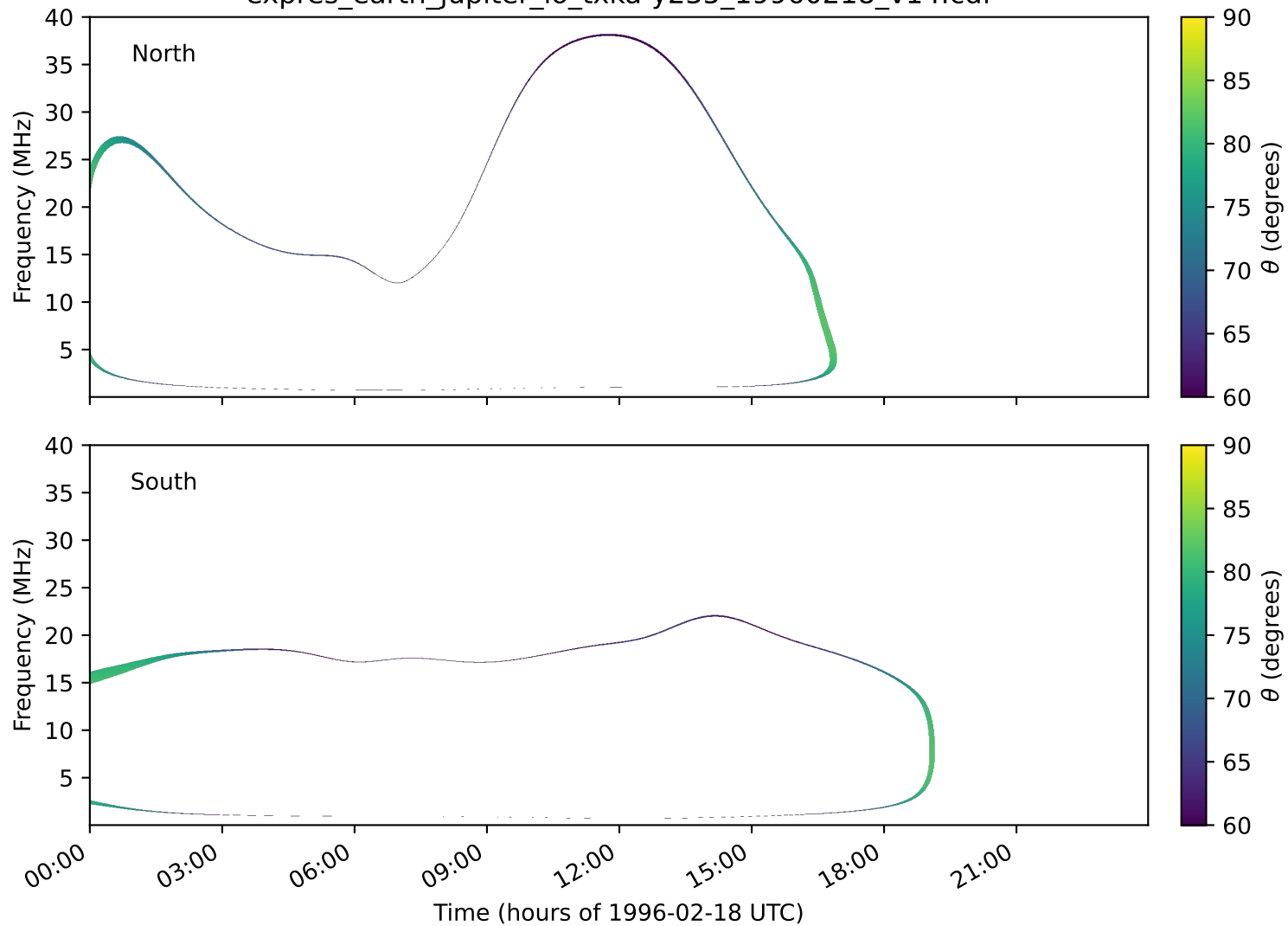
expres_earth_jupiter_io_txka-y235_19960218_v14.cdf
