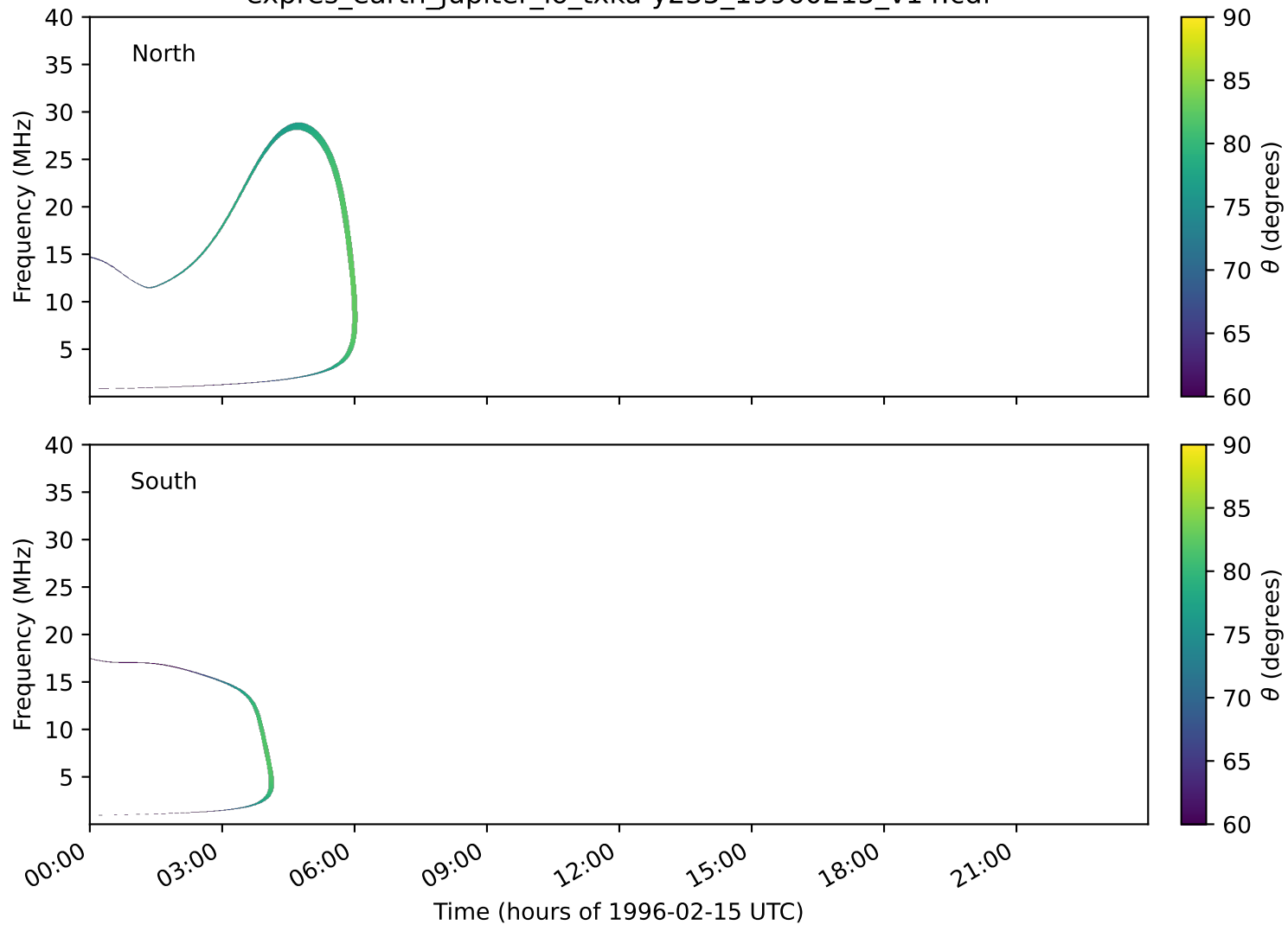
expres_earth_jupiter_io_txka-y235_19960215_v14.cdf
