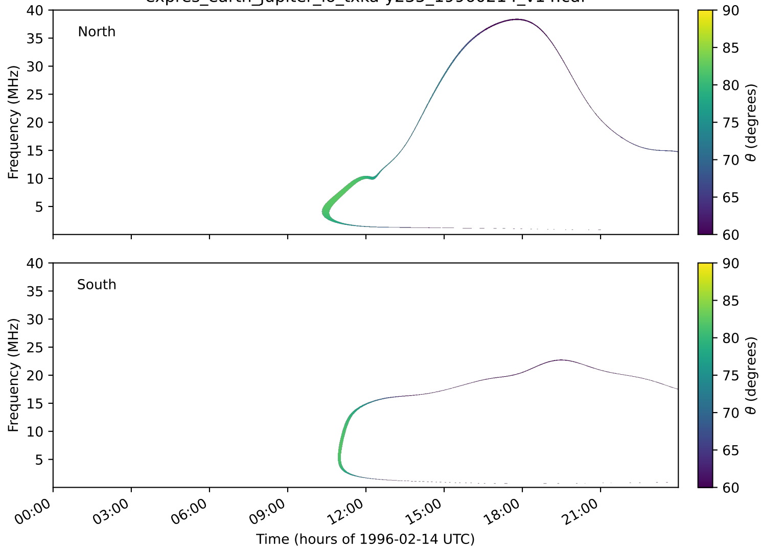
expres_earth_jupiter_io_txka-y235_19960214_v14.cdf
