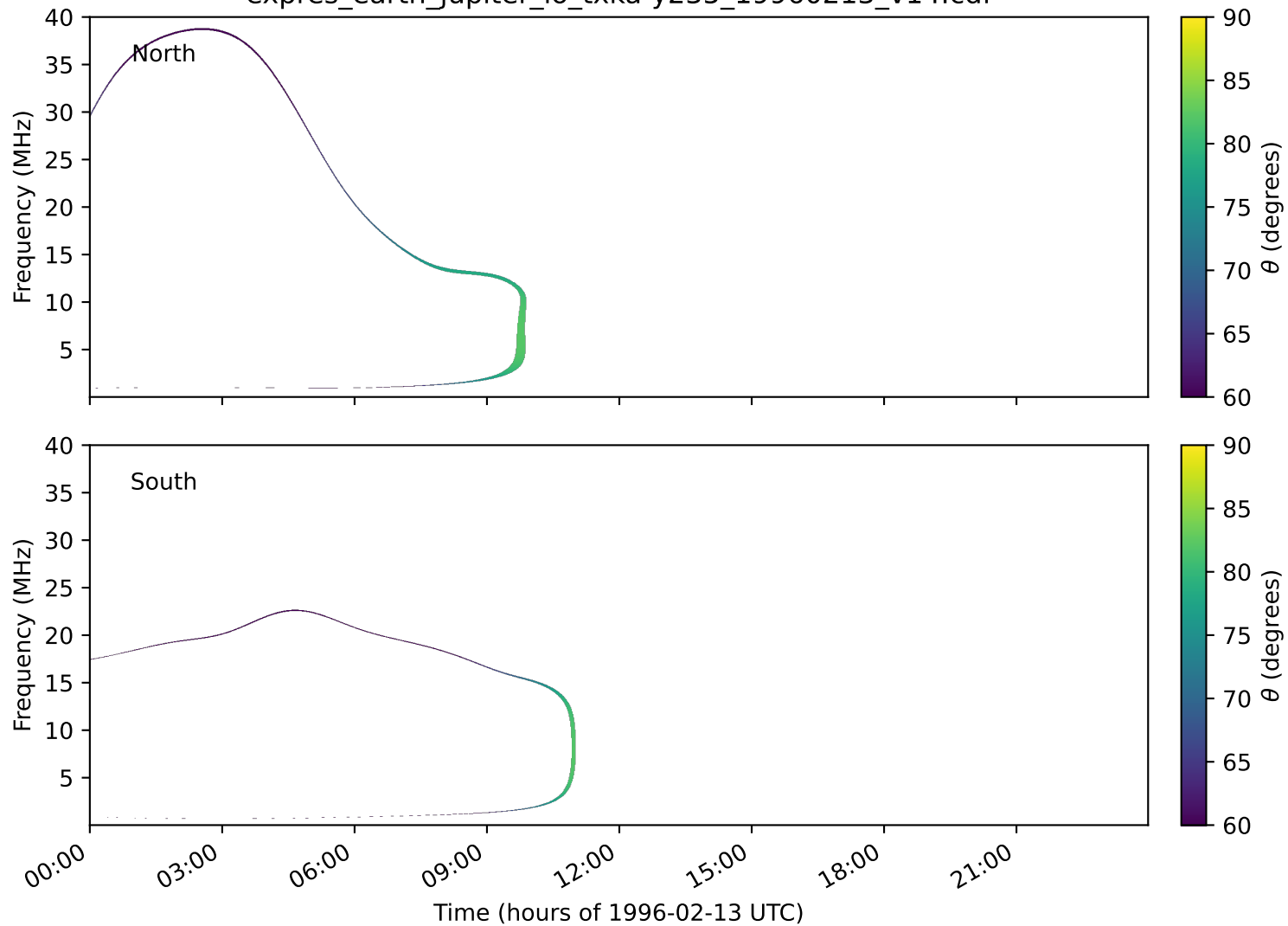
expres_earth_jupiter_io_txka-y235_19960213_v14.cdf
