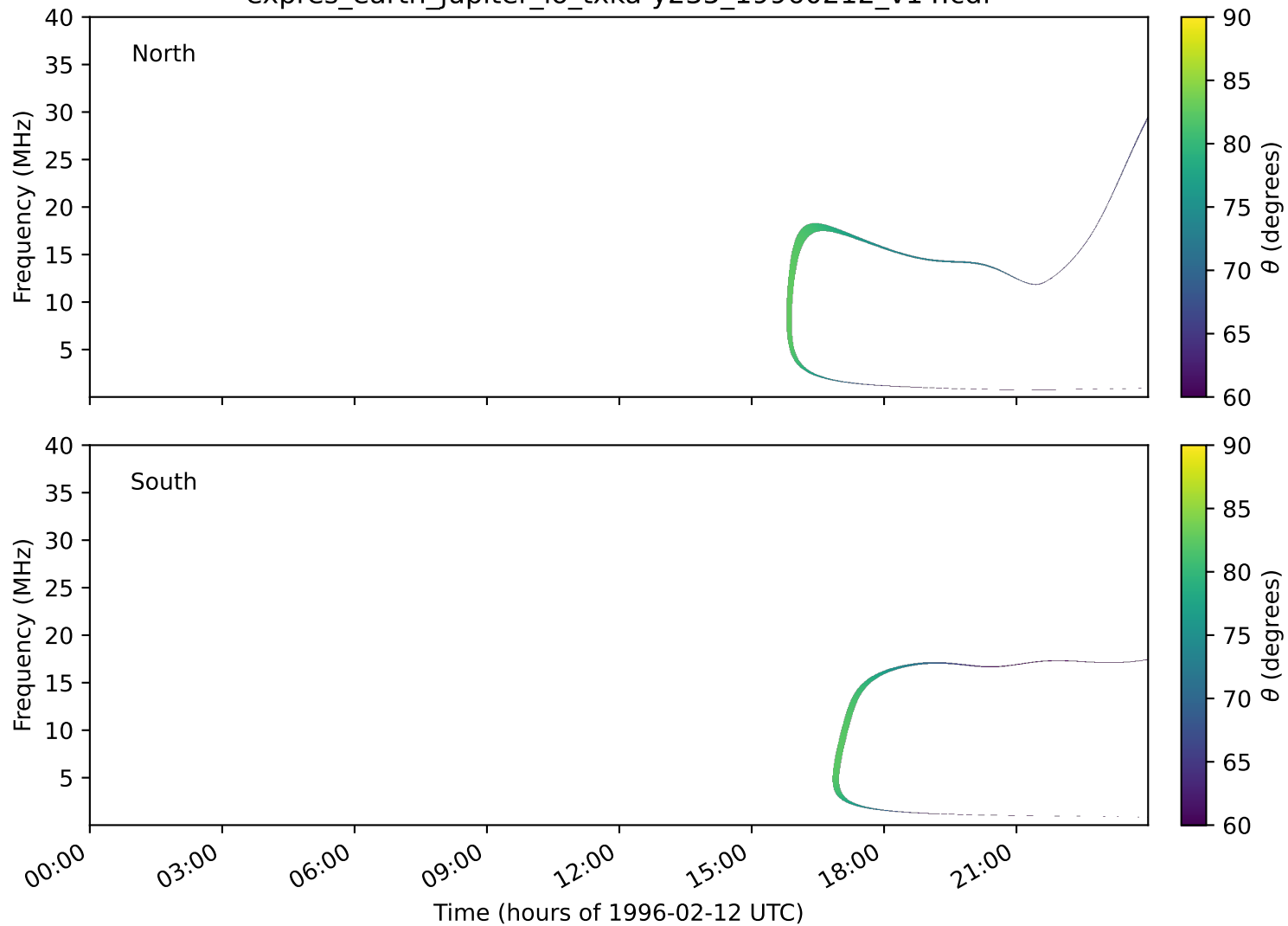
expres_earth_jupiter_io_txka-y235_19960212_v14.cdf
