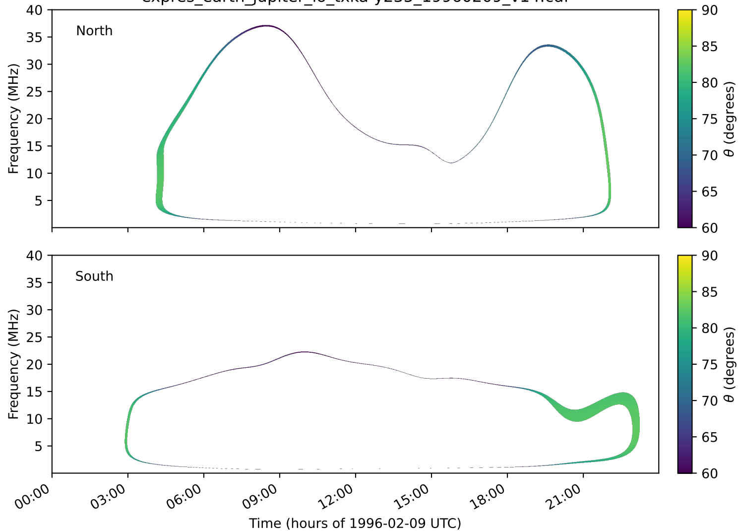
expres_earth_jupiter_io_txka-y235_19960209_v14.cdf
