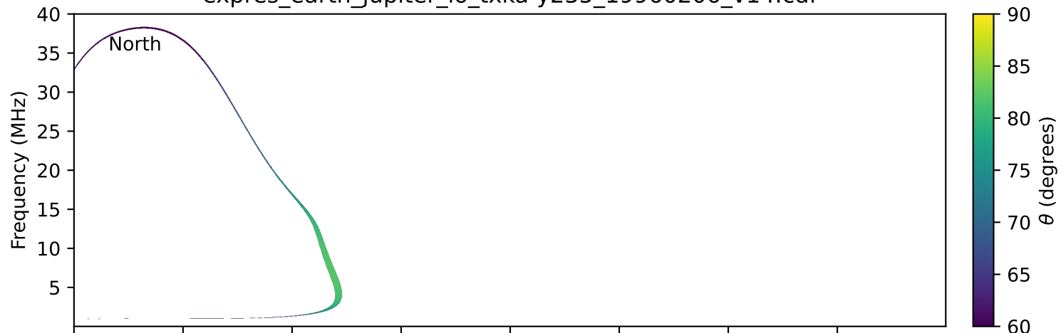
expres_earth_jupiter_io_txka-y235_19960206_v14.cdf
