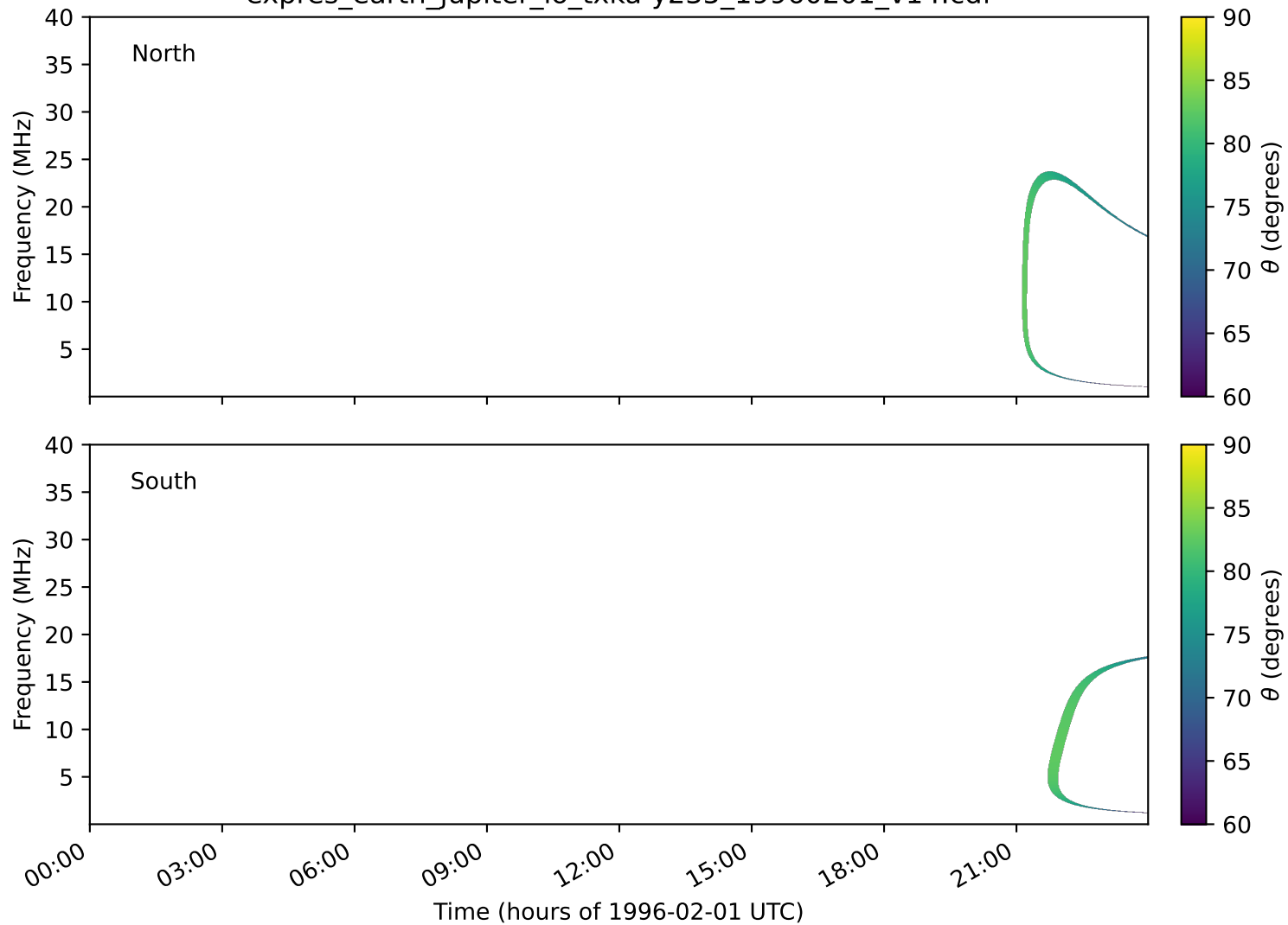
expres_earth_jupiter_io_txka-y235_19960201_v14.cdf
