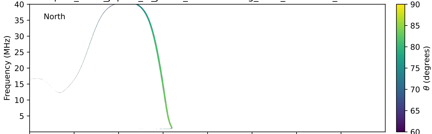
expres_earth_jupiter_io_jrm33_lossc-wid1deg_3kev_19960229_v11.cdf
