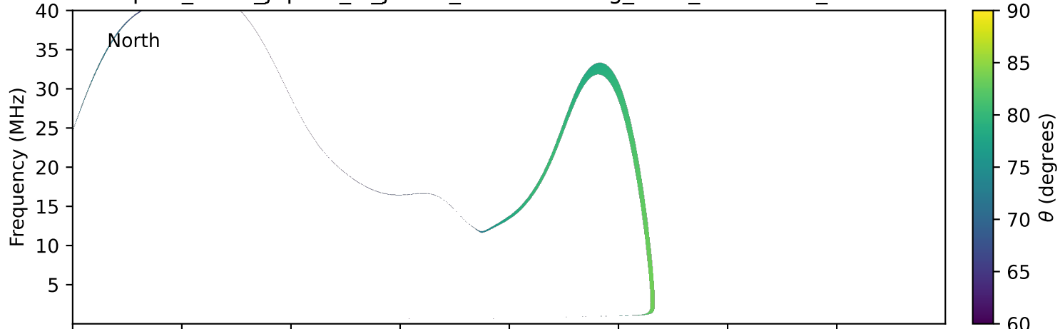
expres_earth_jupiter_io_jrm33_lossc-wid1deg_3kev_19960227_v11.cdf
