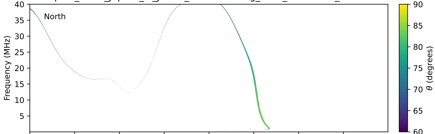
expres_earth_jupiter_io_jrm33_lossc-wid1deg_3kev_19960211_v11.cdf
