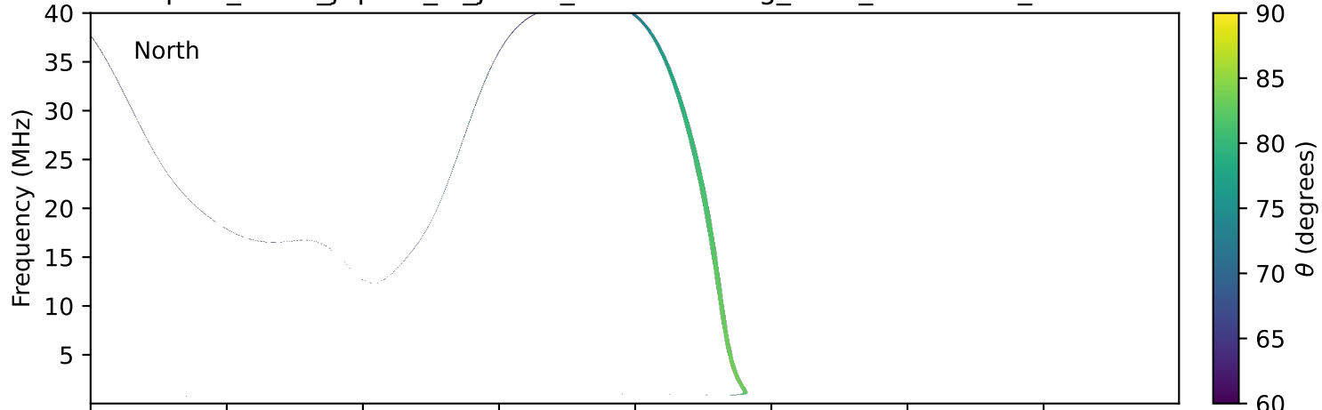
expres_earth_jupiter_io_jrm33_lossc-wid1deg_3kev_19960204_v11.cdf
