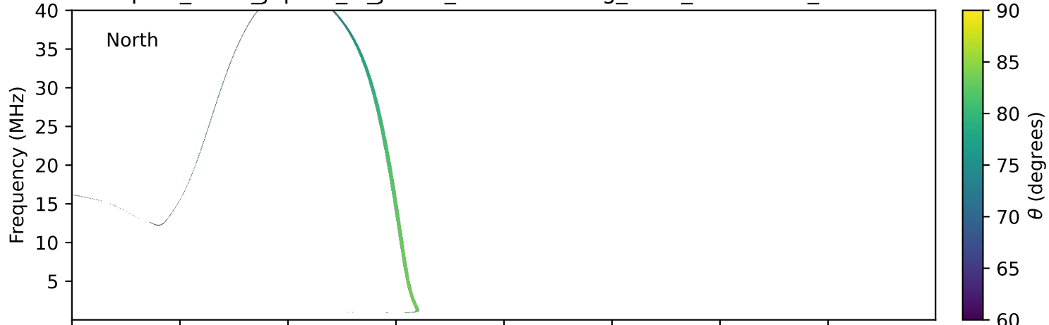
expres_earth_jupiter_io_jrm09_lossc-wid1deg_3kev_19960229_v11.cdf
