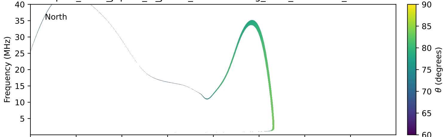
expres_earth_jupiter_io_jrm09_lossc-wid1deg_3kev_19960227_v11.cdf
