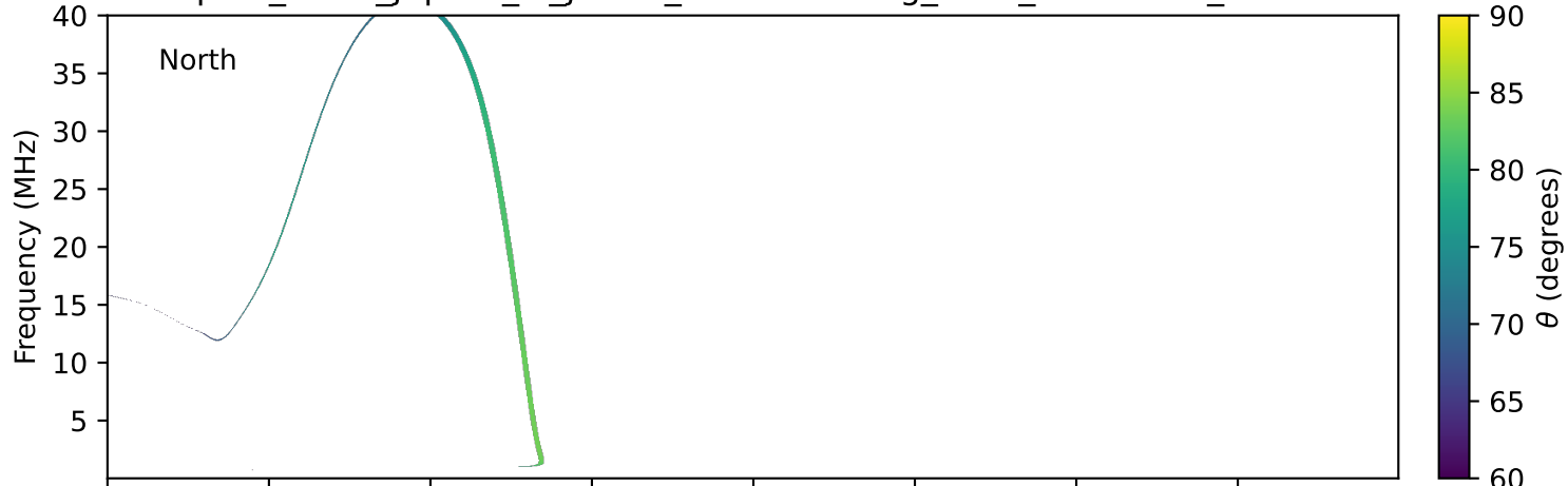
expres_earth_jupiter_io_jrm09_lossc-wid1deg_3kev_19960222_v11.cdf
